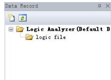
Figure 6.2 data record
